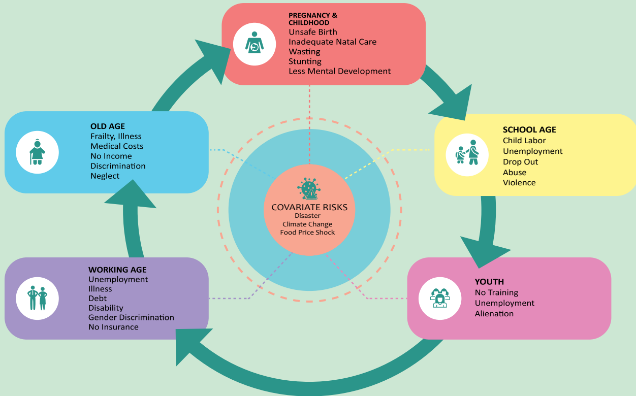
Figure 3: Lifecycle Framework
